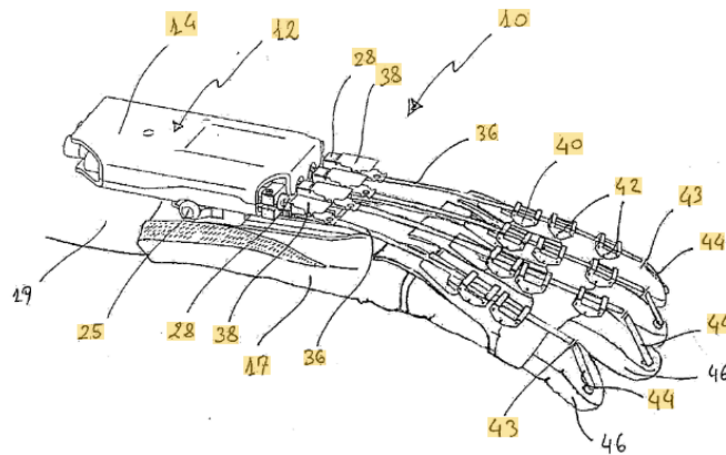
Fig 6.1. Hand rehabilitation device
